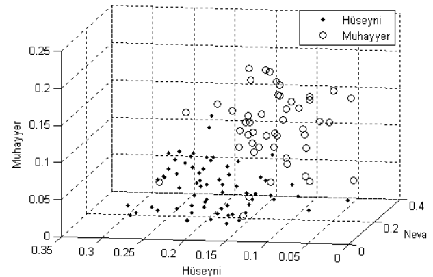
Figure 3. Samples from Hüseyni and Muhayyer classes for the three dimensional feature space: relative frequencies of notes Neva, Hüseyni and Muhayyer.
