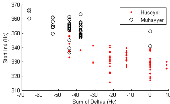
Figure 9. Seyir features: starting region and sum of deltas for makams Muhayyer and Hüseyni .
