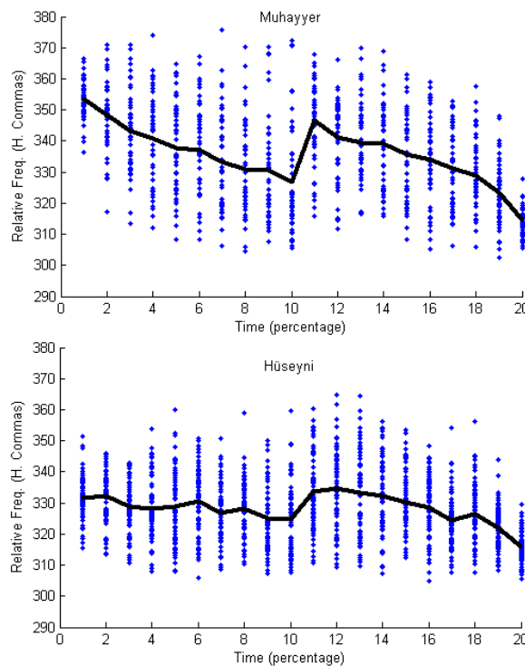
Figure 8. Melodic progression of makam Muhayyer and Hüseyni (from symbolic data).
