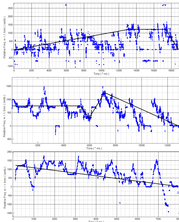
Figure 6. Melographs from three makams: Uşşak (taksim of Yorgo Bacanos), Hüseyni (taksim of Fahrettin Çimenli), Muhayyer (taksim of İhsan Özgen).
