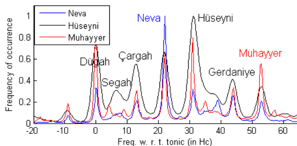
Figure 1. Pitch histogram templates of three makams: Neva , Hüseyni and Muhayyer . Names written close to the peaks correspond to note ( perde ) names.
